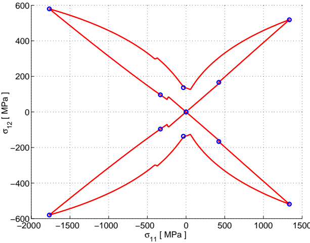
Figure 9: Tension torsion test: numerical results (in terms of stress \sigma_{11} versus stress \sigma_{12} ) for two different time discretizations.
