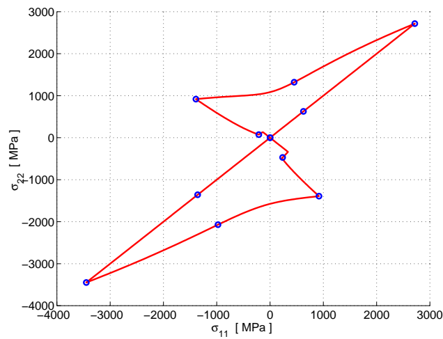
Figure 7: Biaxial tension test: numerical results (in terms of stress \sigma_{11} versus stress \sigma_{22} ) for two different time discretizations.
