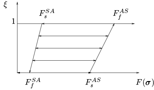
Figure 1: Diagram of relation g , expressing the dependency of the material fraction \xi on the general loading function F(\boldsymbol{\sigma}) .
