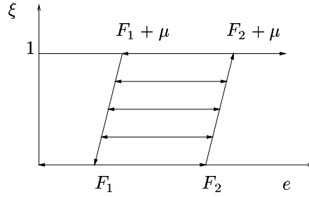
Figure 3: Diagram of relation q , expressing the dependency of the material fraction \xi on the strain measure e
