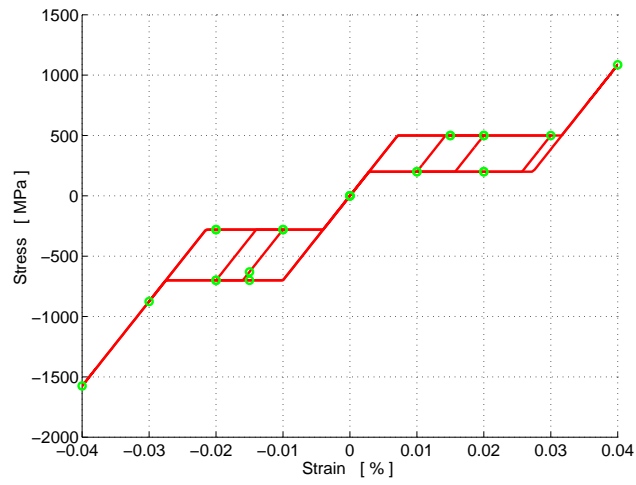
Figure 6: Uniaxial tension test: numerical results (in terms of stress versus strain) for two different time discretizations.
