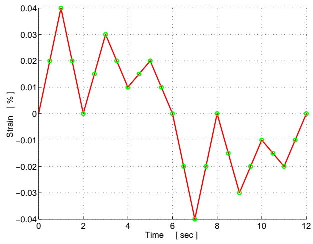
Figure 4: Uniaxial tension test: loading history in terms of strain versus time for two different time discretizations.
