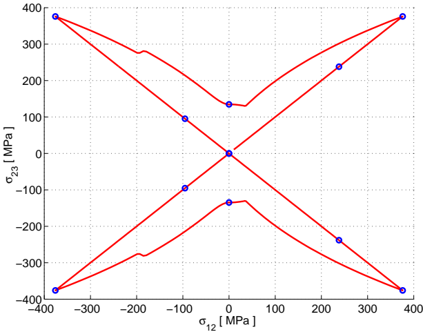
Figure 8: Biaxial torsion test: numerical results (in terms of stress \sigma_{12} versus stress \sigma_{23} ) for two different time discretizations.
