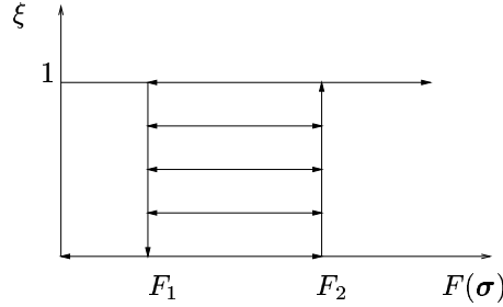
Figure 2: Diagram of relation g , expressing the dependency of the material fraction \xi on the general loading function F(\sigma) , for the case of no hardening.
