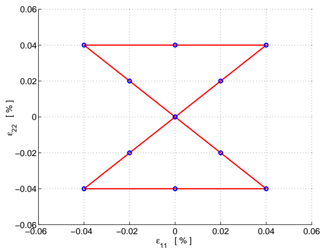
Figure 5: Biaxial test: loading history (in terms of strain \epsilon_{11} versus strain \epsilon_{22} ) for two different time discretizations.
